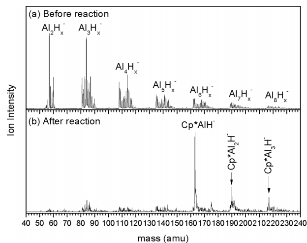
FIG. 1. (a) Mass spectrum of aluminum hydride cluster anions before reaction and (b) mass spectrum of \text{Cp}^*\text{Al}_{1-3}\text{H}^- cluster anions after reaction.
